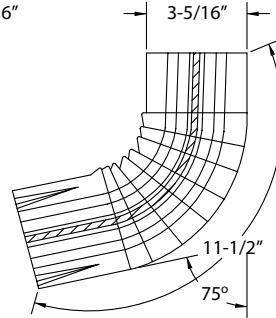
ABE23 B-Elbow
